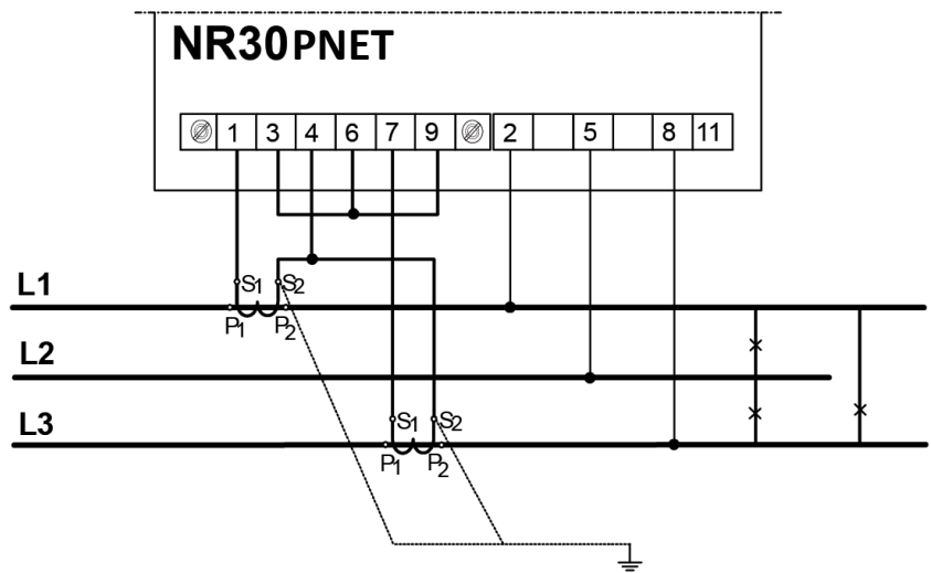
Fig.5. Input signal connection in 3-phase 3 - wire network
